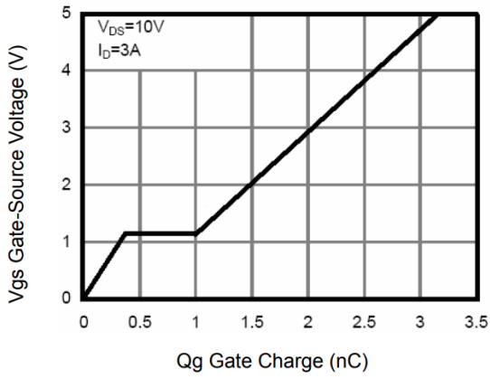
Gate-Charge Characteristic
