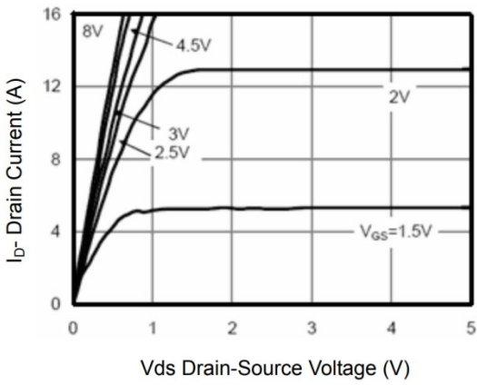
Output Characteristic
