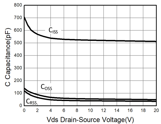
Capacitance Characteristic
