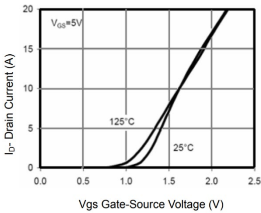
Transfer Characteristic
