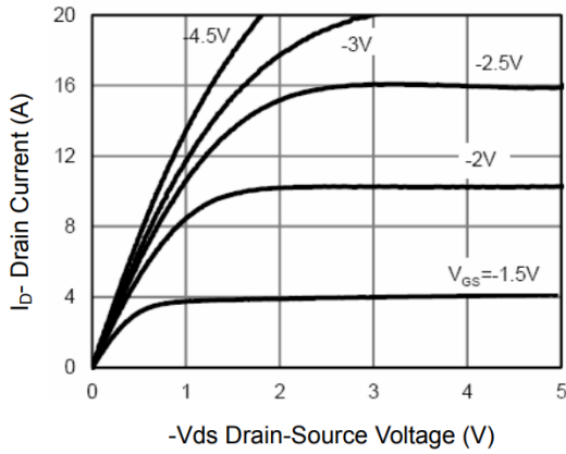
Output Characteristic
