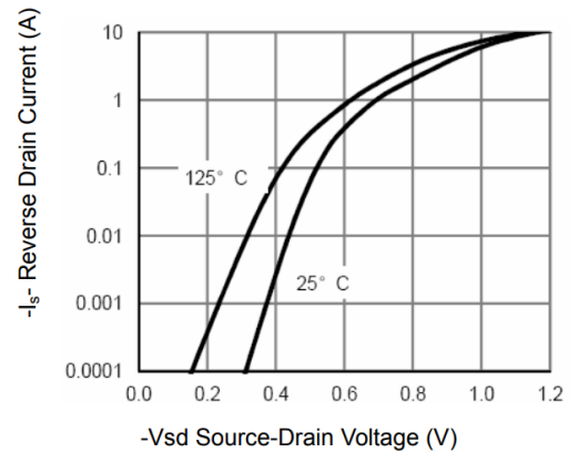
Body Diode Characteristic
