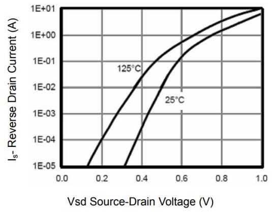
Body Diode Characteristic
