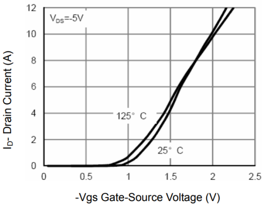
Transfer Characteristic
