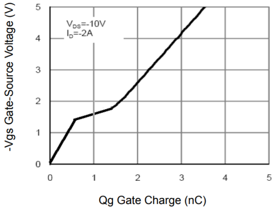
Gate-Charge Characteristic
