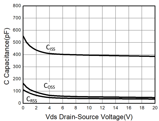
Capacitance Characteristic
